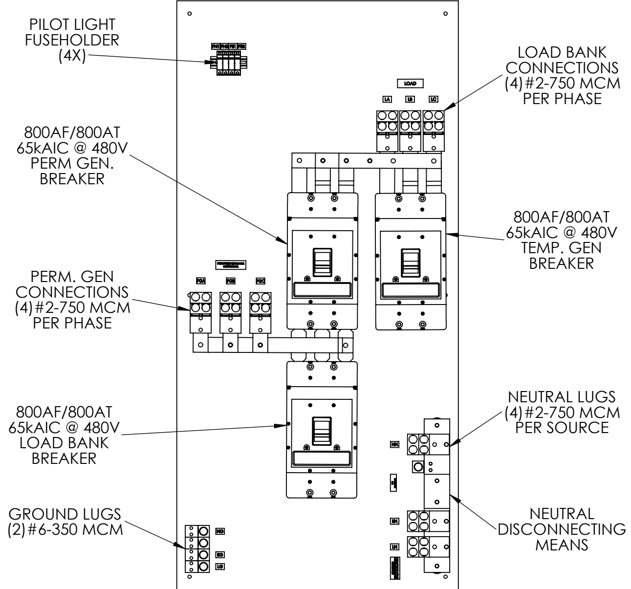
FRONT VIEW (ENCLOSURE REMOVED)
