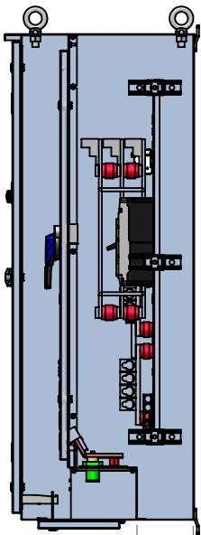
RIGHT SIDE (CUTAWAY)
