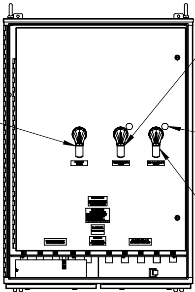
FRONT VIEW (FIRST DOOR REMOVED)
