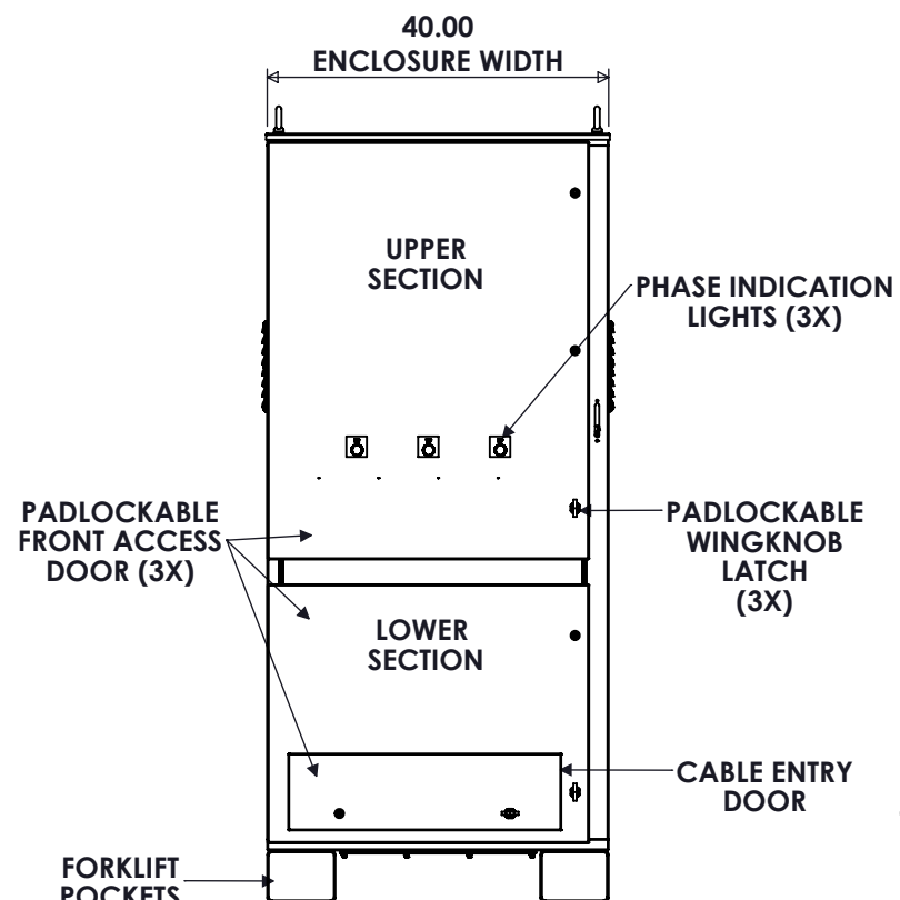
FRONT VIEW
