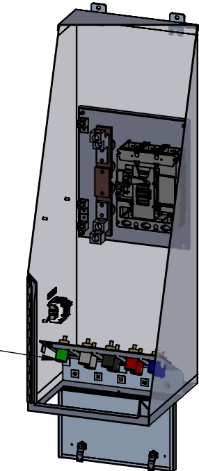
INTERIOR TRIMETRIC VIEW
