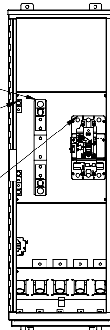
FRONT VIEW (DOORS REMOVED)
