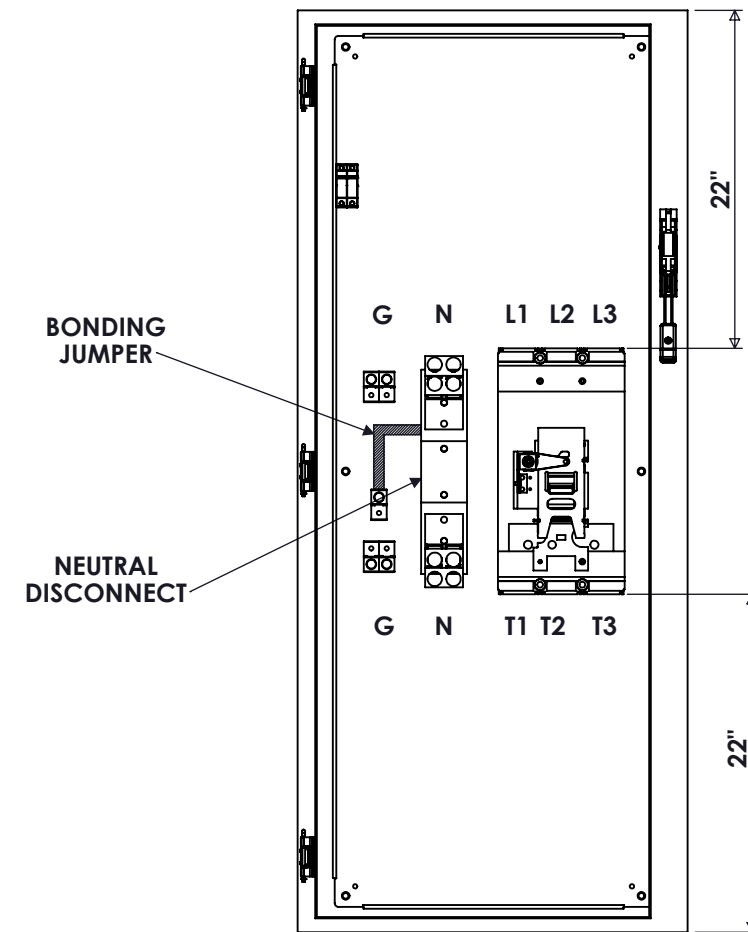
FRONT VIEW DOOR REMOVED
