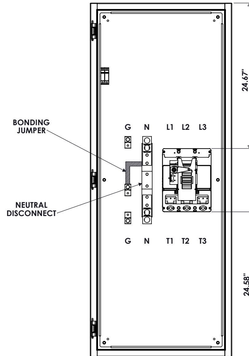
FRONT VIEW DOOR REMOVED
