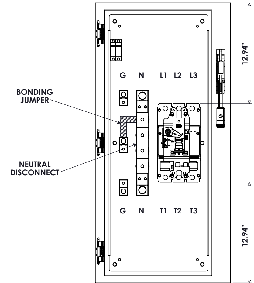
FRONT VIEW DOOR REMOVED
