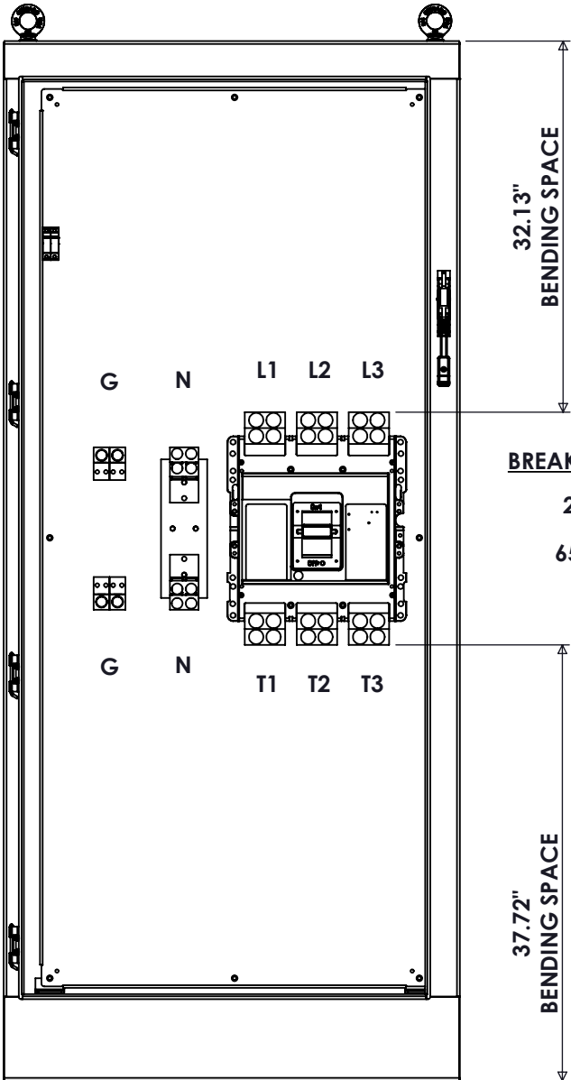
FRONT VIEW DOOR REMOVED
