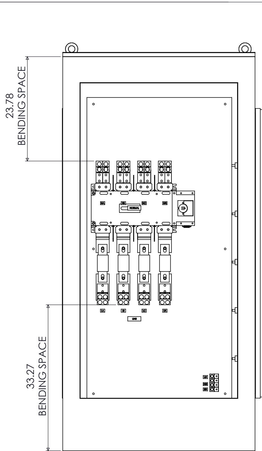
FRONT VIEW DOOR REMOVED
