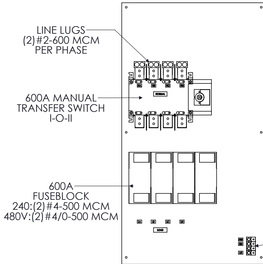
FRONT VIEW ENCLOSURE REMOVED
