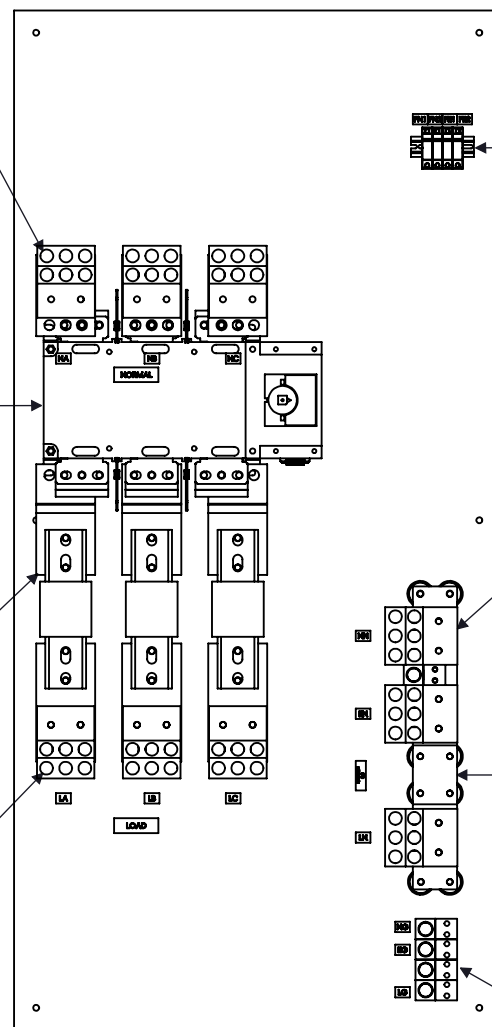
FRONT VIEW ENCLOSURE REMOVED
