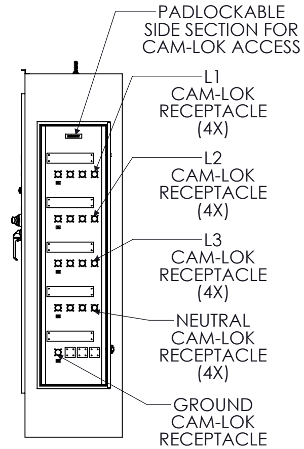
SIDE VIEW
