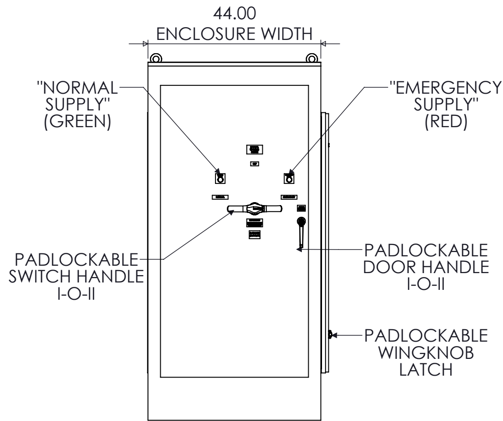
FRONT VIEW
