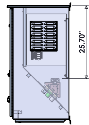
SIDE VIEW INTERIOR
