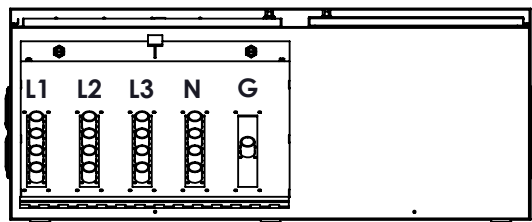
BOTTOM VIEW DOOR REMOVED
