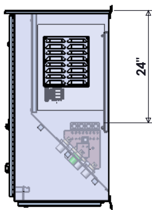
SIDE VIEW INTERIOR
