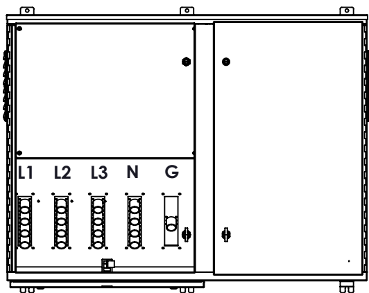
FRONT VIEW DOOR REMOVED
