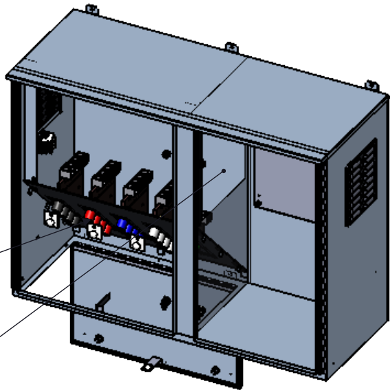
TRIMETRIC VIEW INTERIOR
