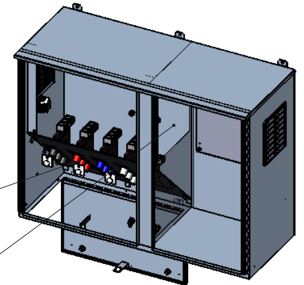
TRIMETRIC VIEW INTERIOR
