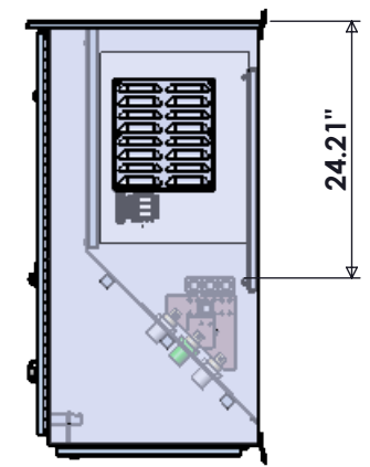
SIDE VIEW INTERIOR
