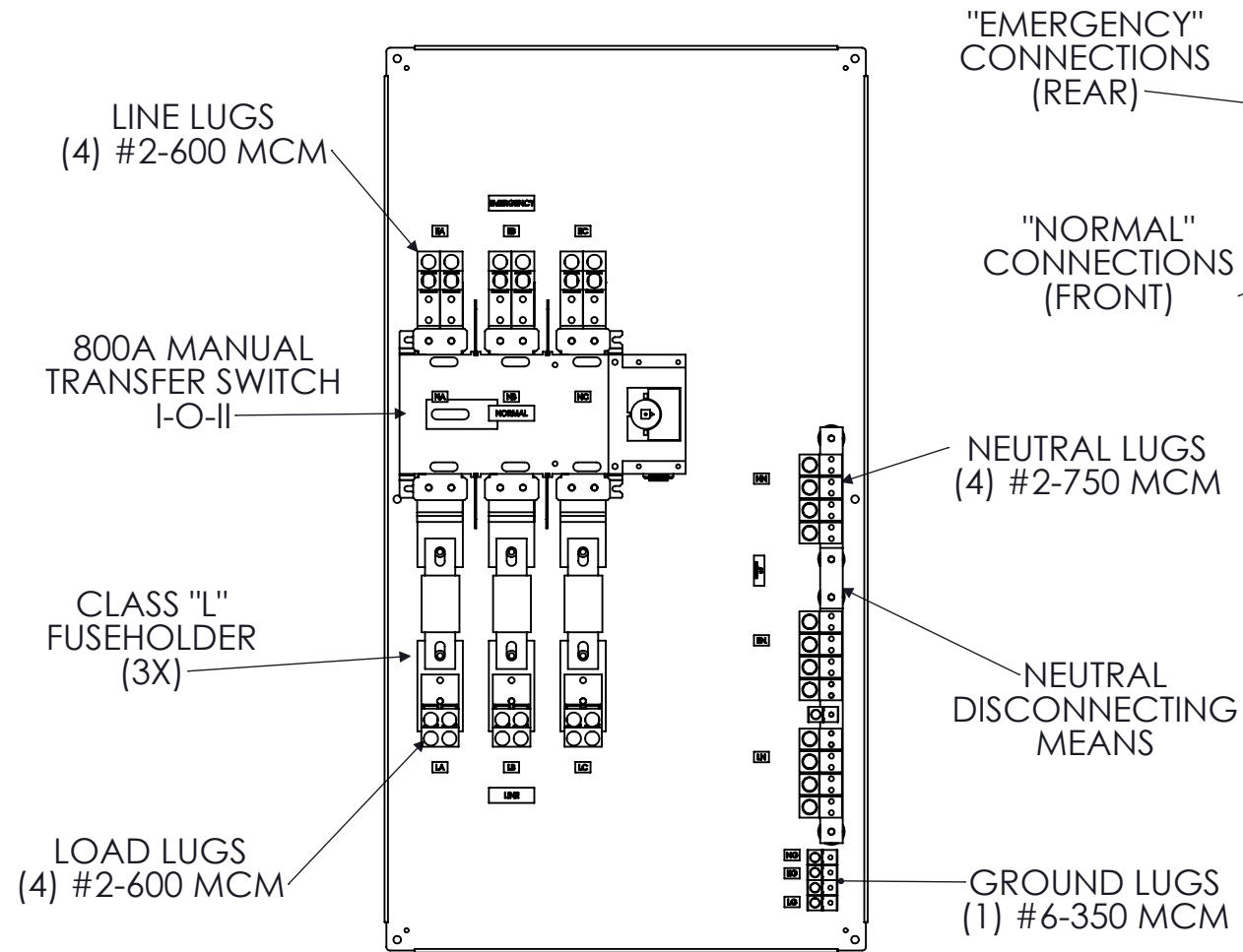
FRONT VIEW ENCLOSURE REMOVED
