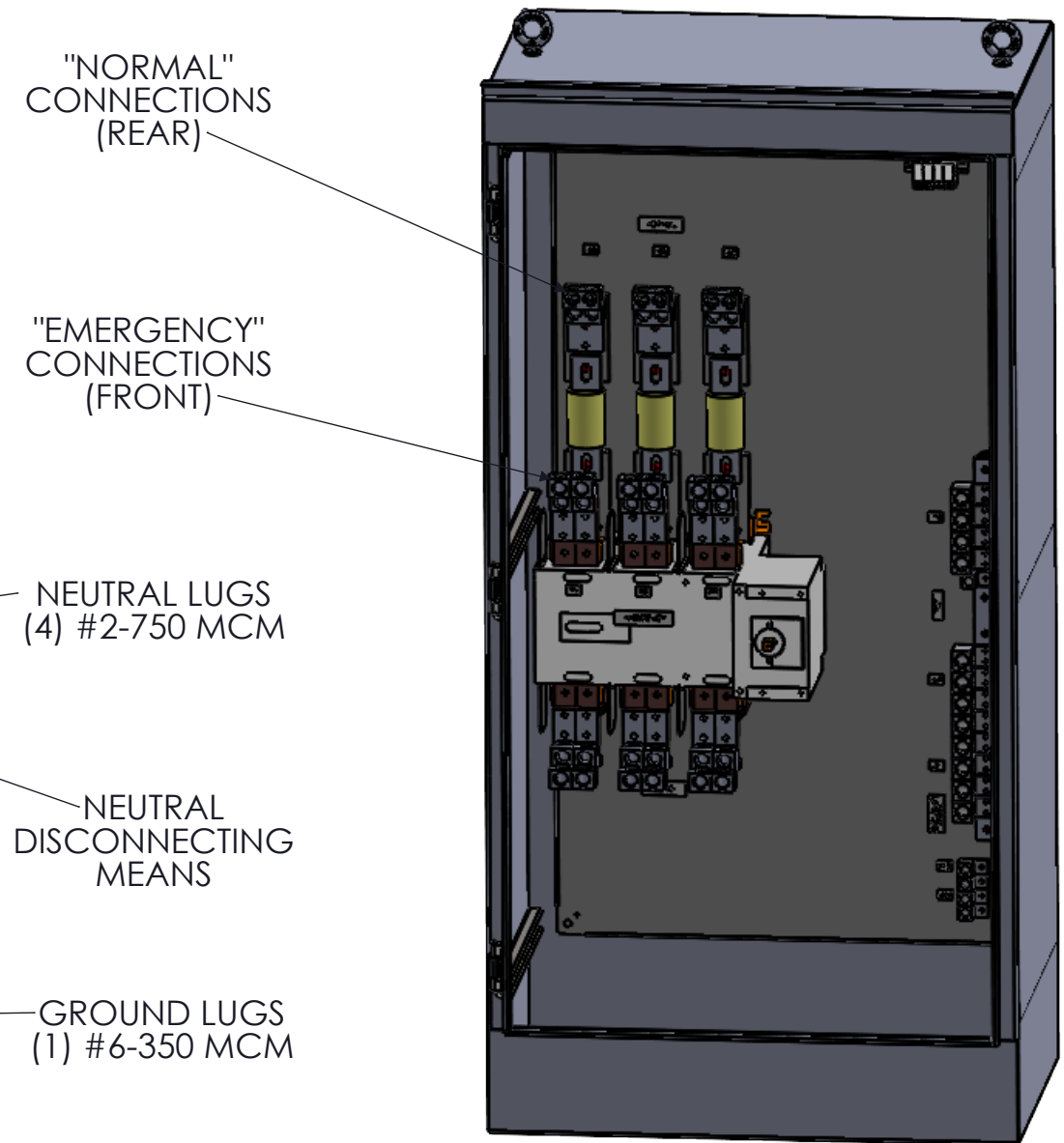
DIMETRIC VIEW DOOR REMOVED
