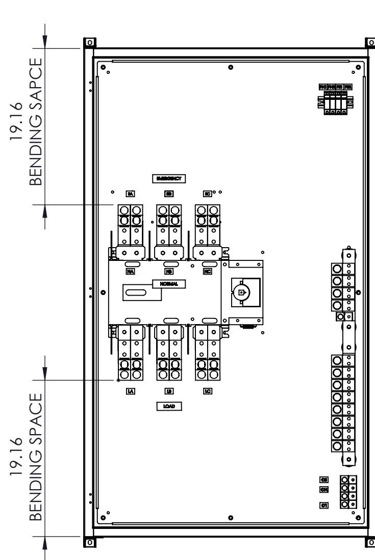
FRONT VIEW DOOR REMOVED
