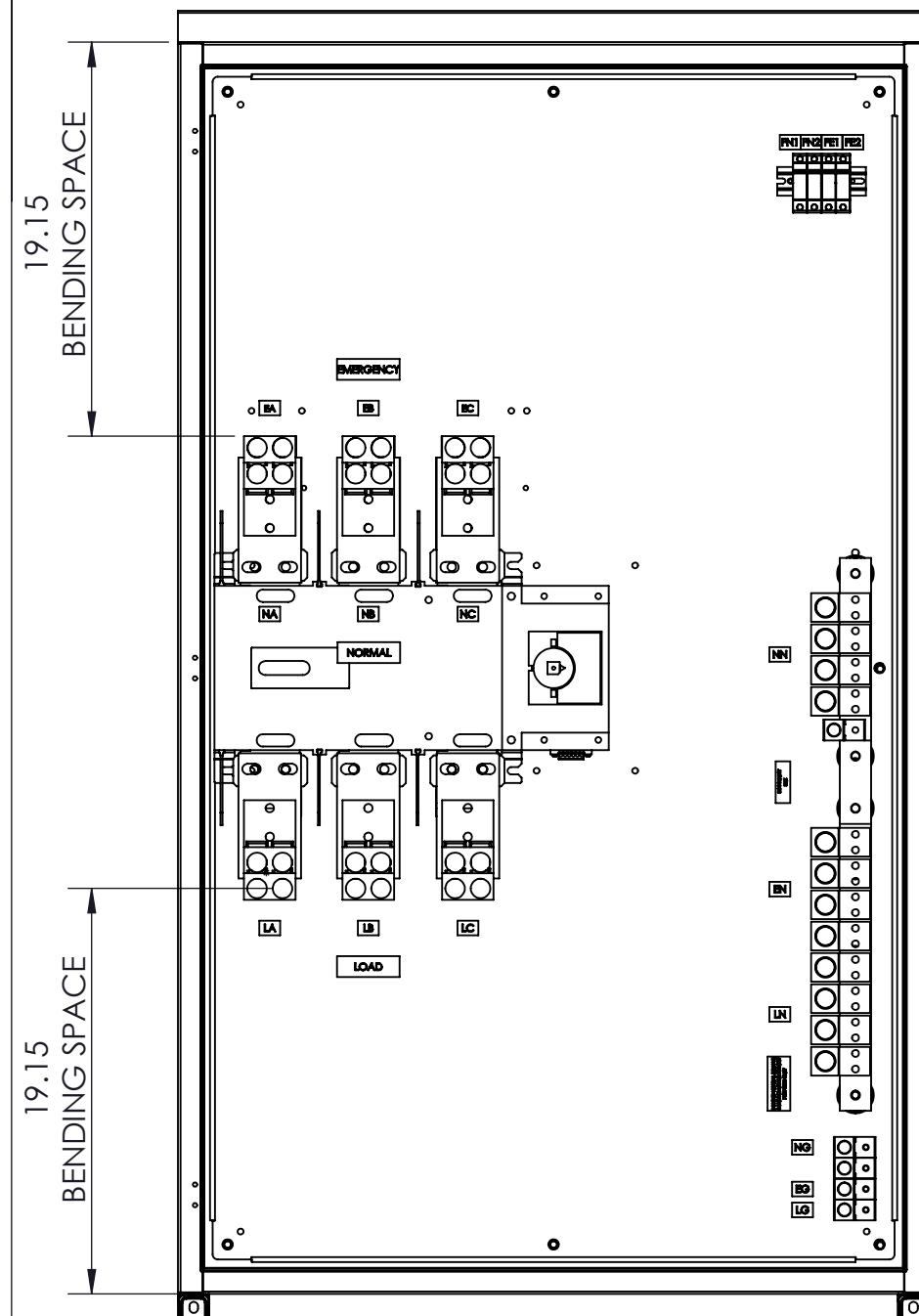
FRONT VIEW DOOR REMOVED
