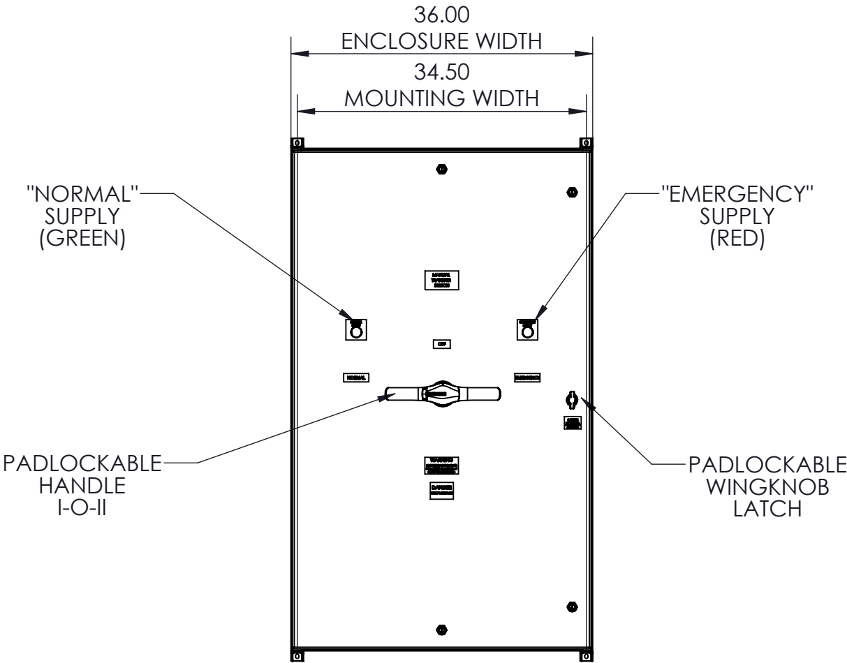
FRONT VIEW
