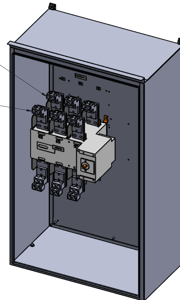
FRONT VIEW DOOR REMOVED
