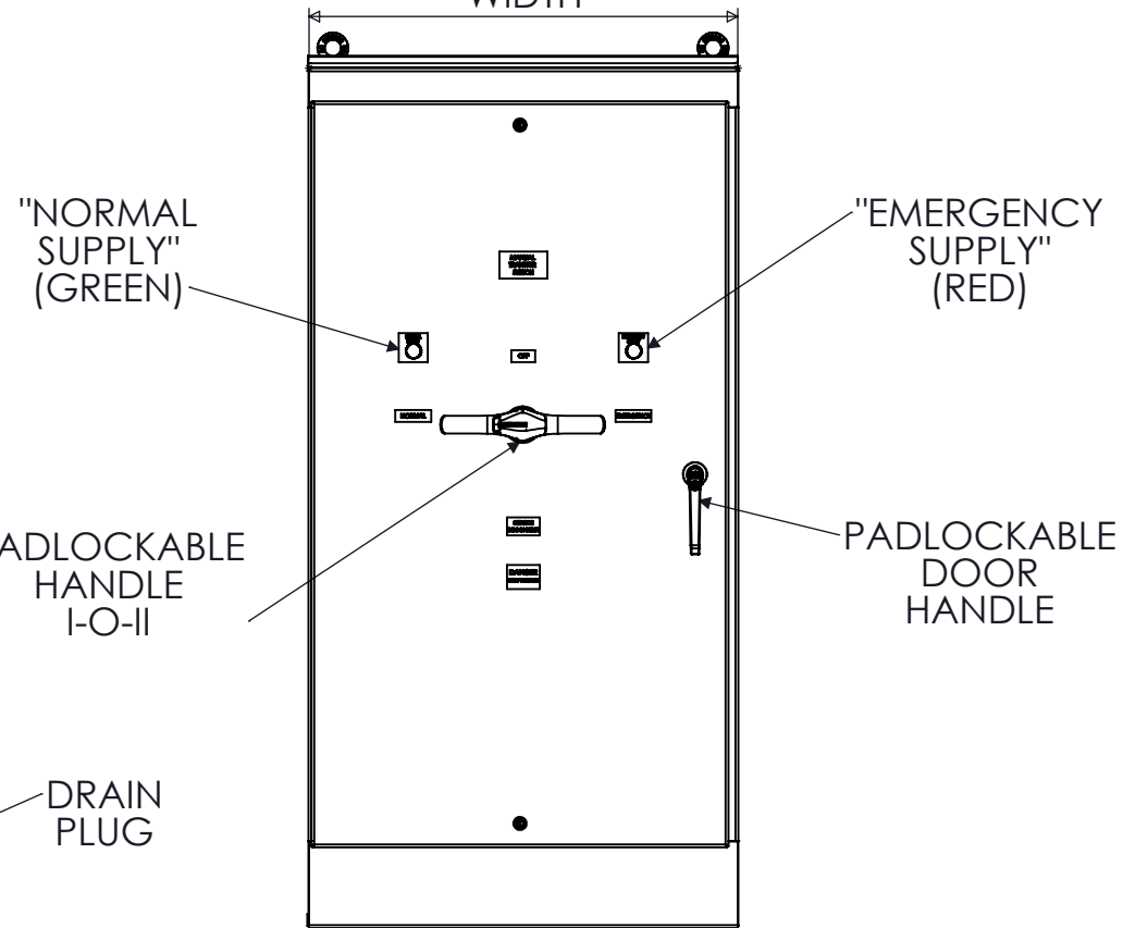
FRONT VIEW
