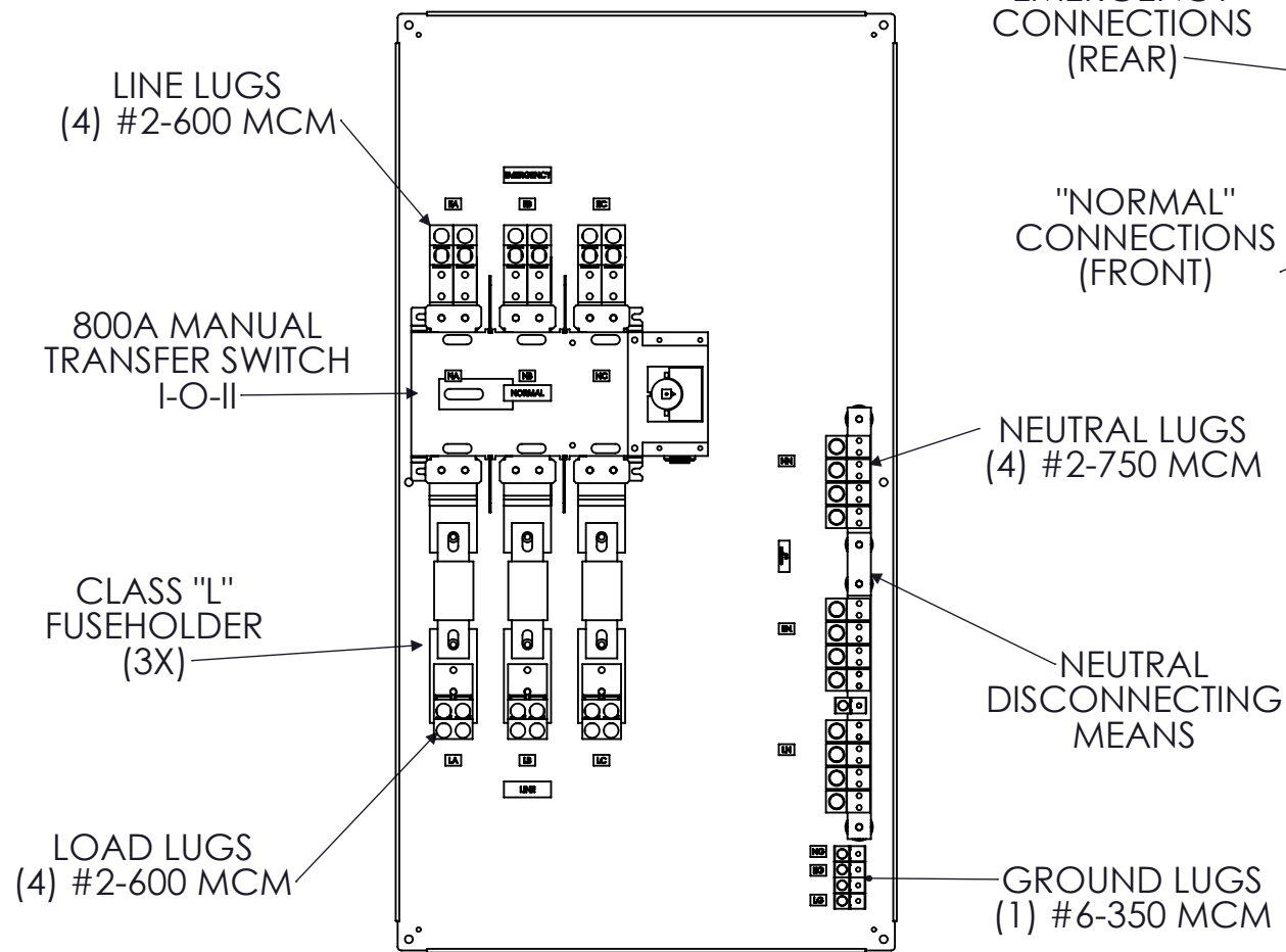
FRONT VIEW ENCLOSURE REMOVED
