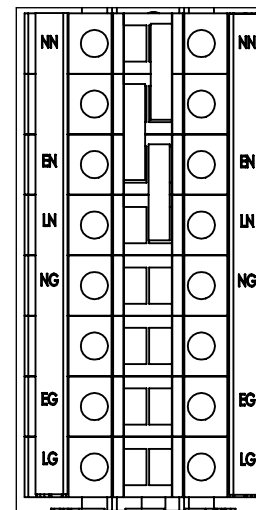
TERMINAL LAYOUT "B"
