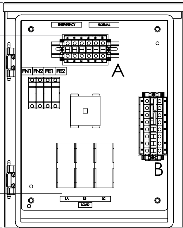
FRONT VIEW DOOR REMOVED
