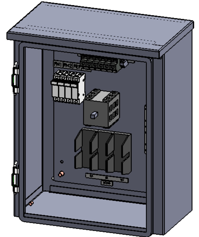
DIMETRIC VIEW DOOR REMOVED
