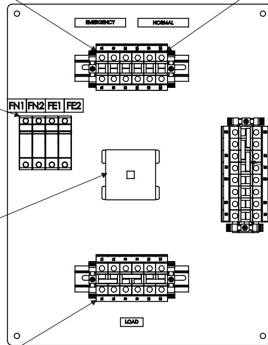
FRONT VIEW ENCLOSURE REMOVED
