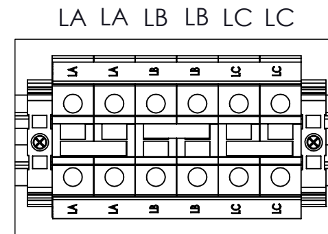
TERMINAL LAYOUT "C"
