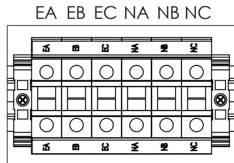
TERMINAL LAYOUT "A"
