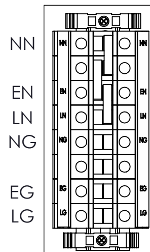
TERMINAL LAYOUT "B"
