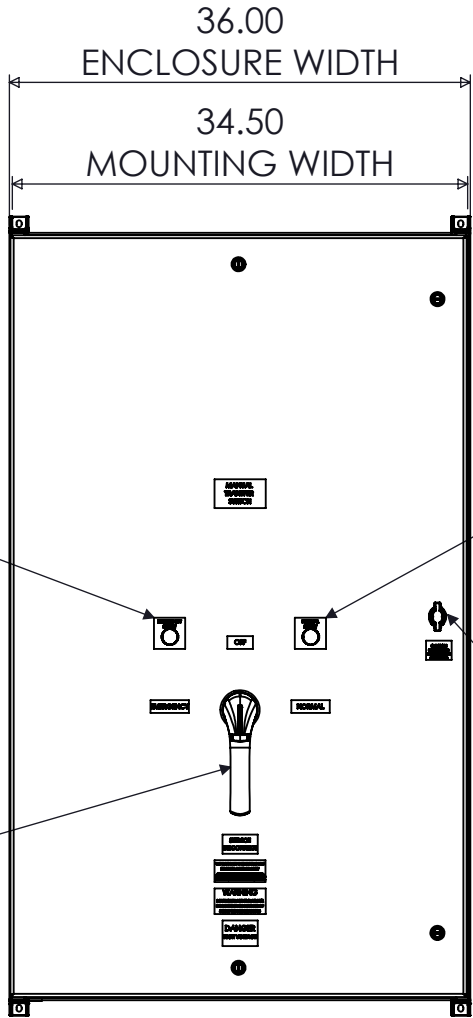
FRONT VIEW
