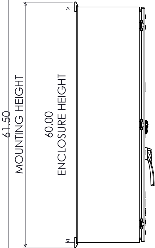
SIDE VIEW
