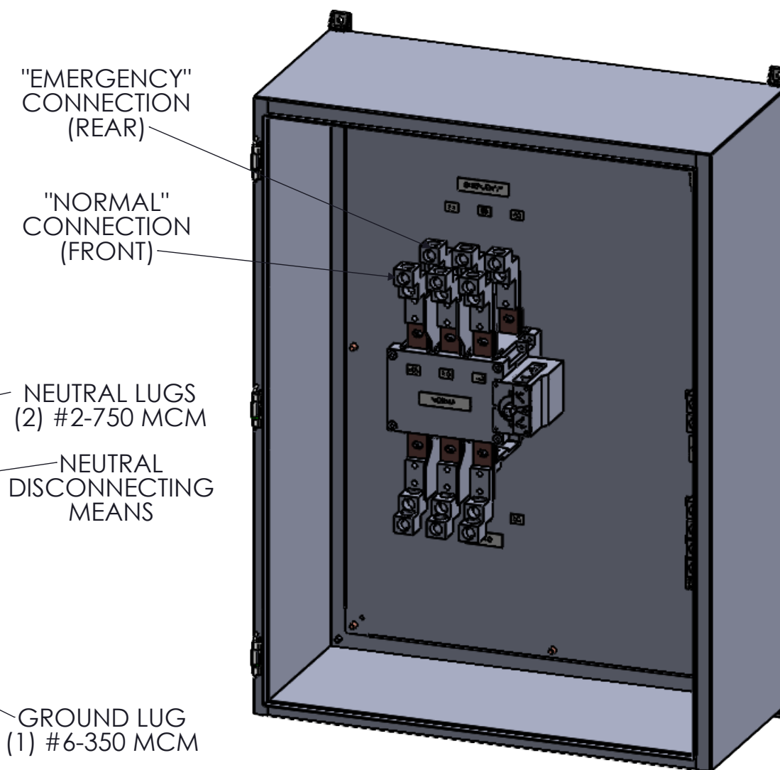
DIMETRIC VIEW DOOR REMOVED
