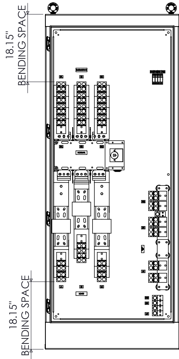
FRONT VIEW DOOR REMOVED
