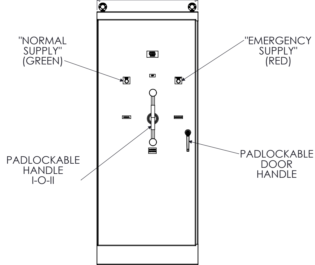
FRONT VIEW
