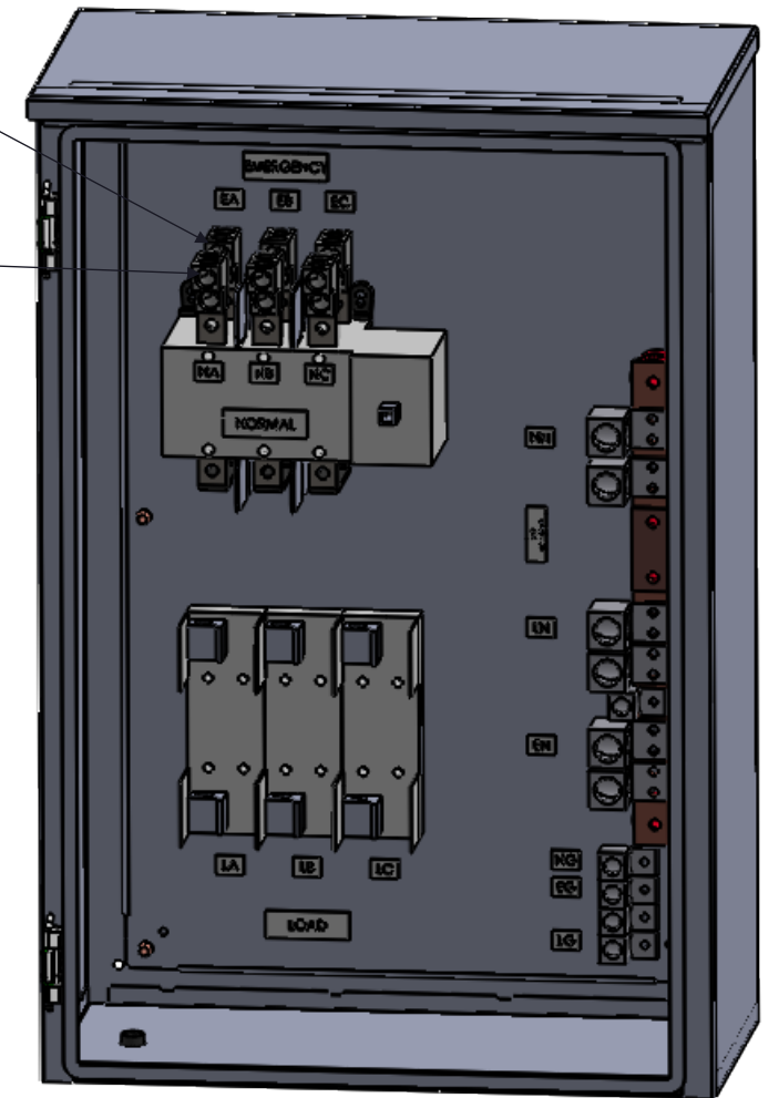
DIMETRIC VIEW DOOR REMOVED
