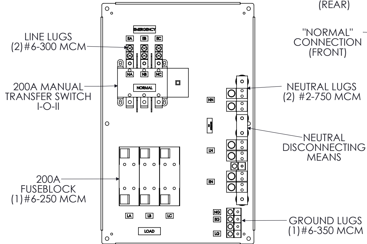
FRONT VIEW ENCLOSURE REMOVED
