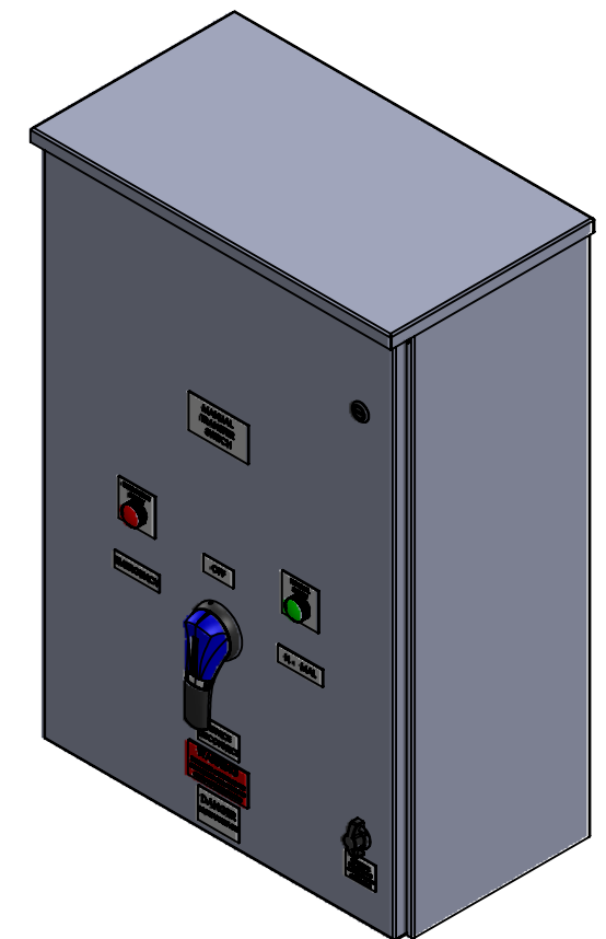
DIMETRIC VIEW
