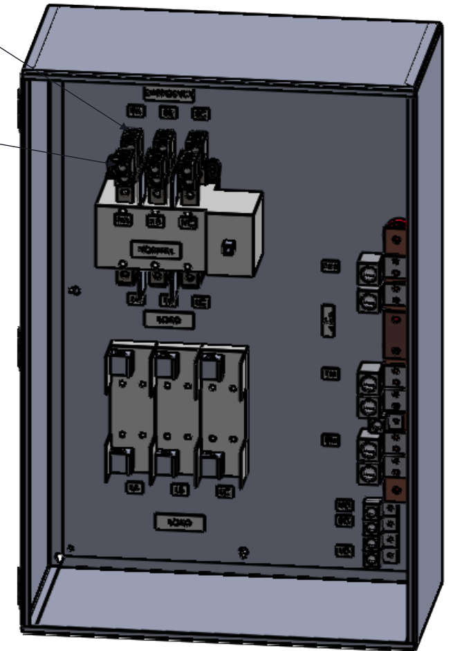
DIMETRIC VIEW
