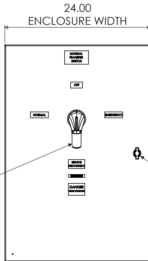
FRONT VIEW
