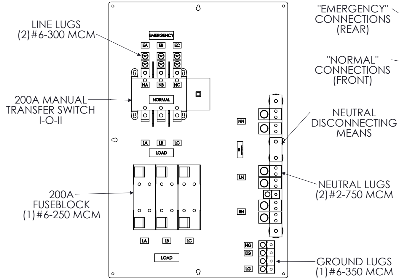
FRONT VIEW
