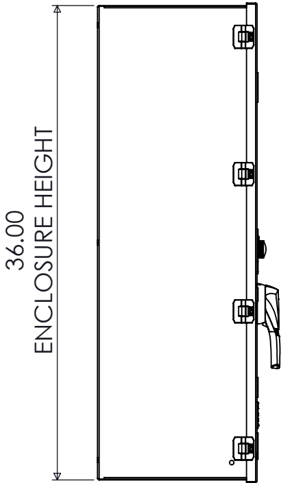
LEFT VIEW
