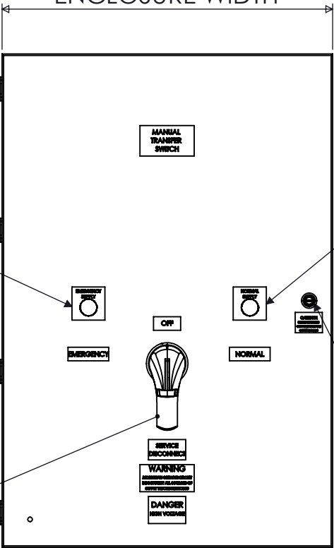
FRONT VIEW
