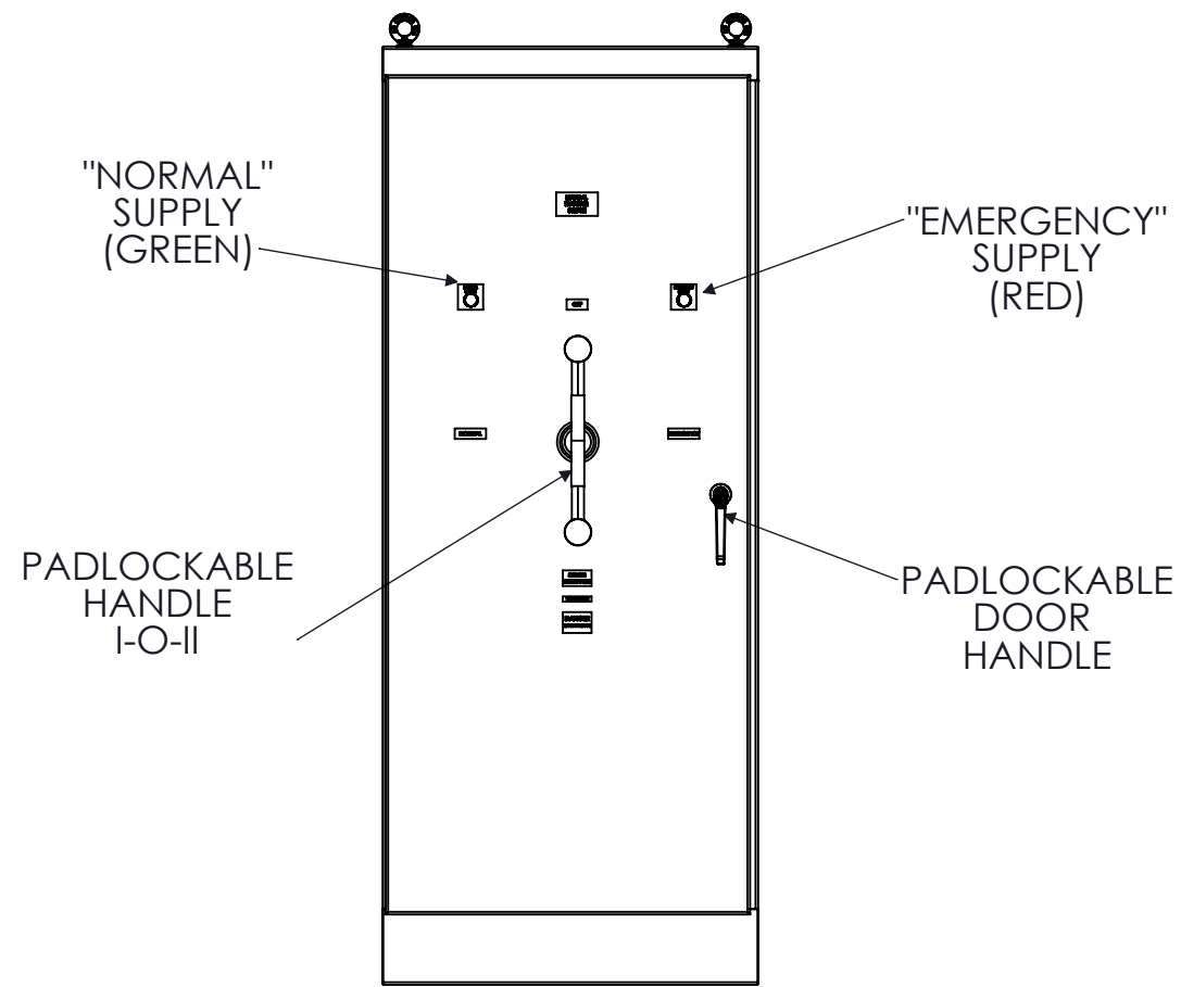
FRONT VIEW
