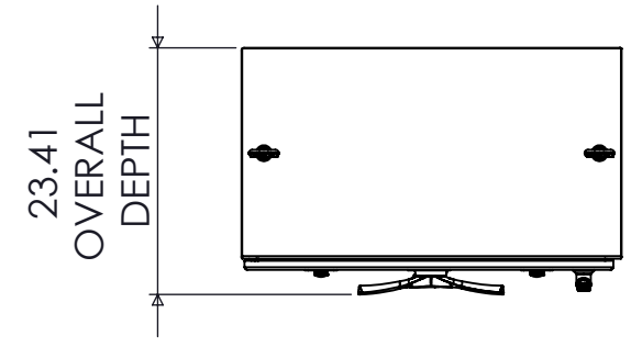
TOP VIEW 36.00 ENCLOSURE WIDTH
