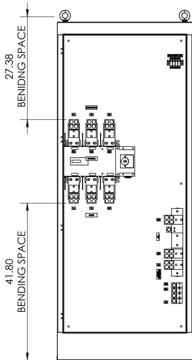
FRONT VIEW
