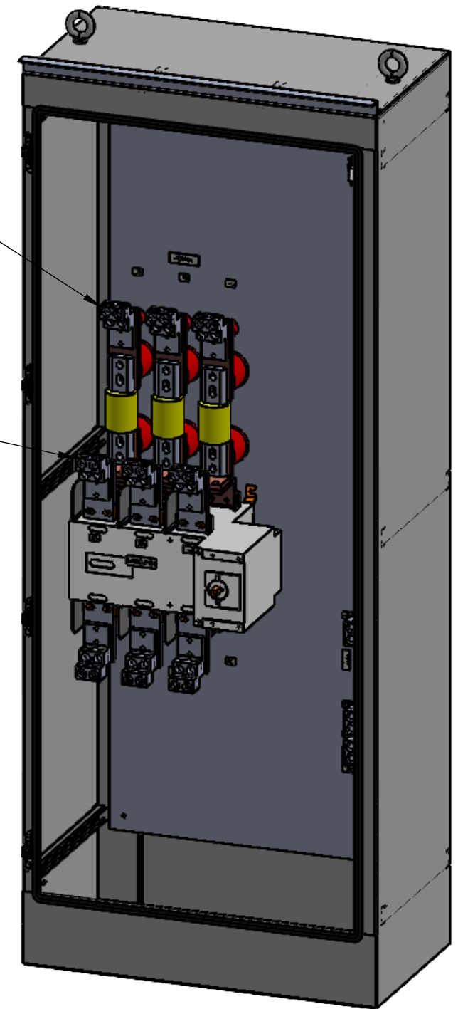
ISOMETRIC VIEW (DOOR REMOVED)
