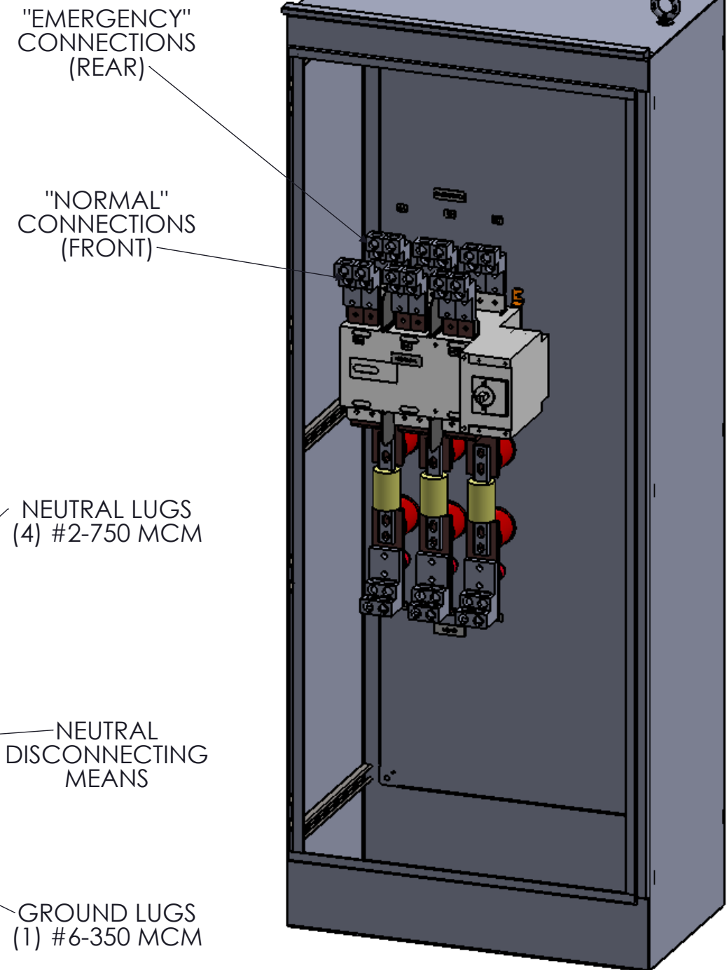
DIMETRIC VIEW DOOR REMOVED
