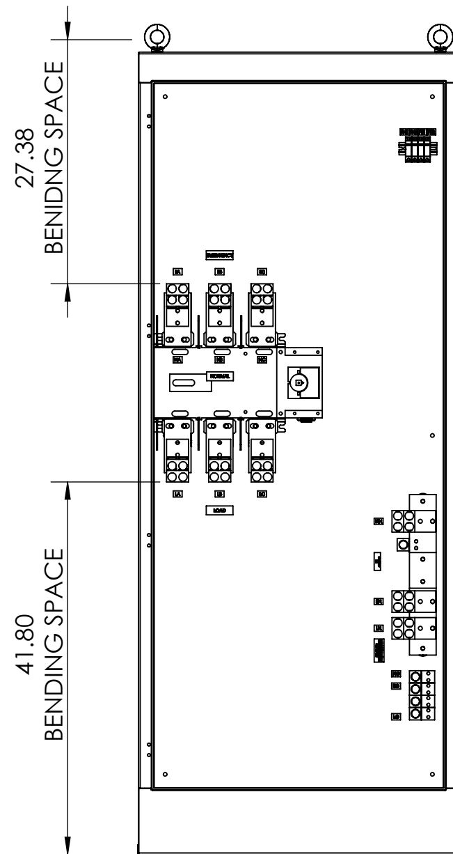
FRONT VIEW
