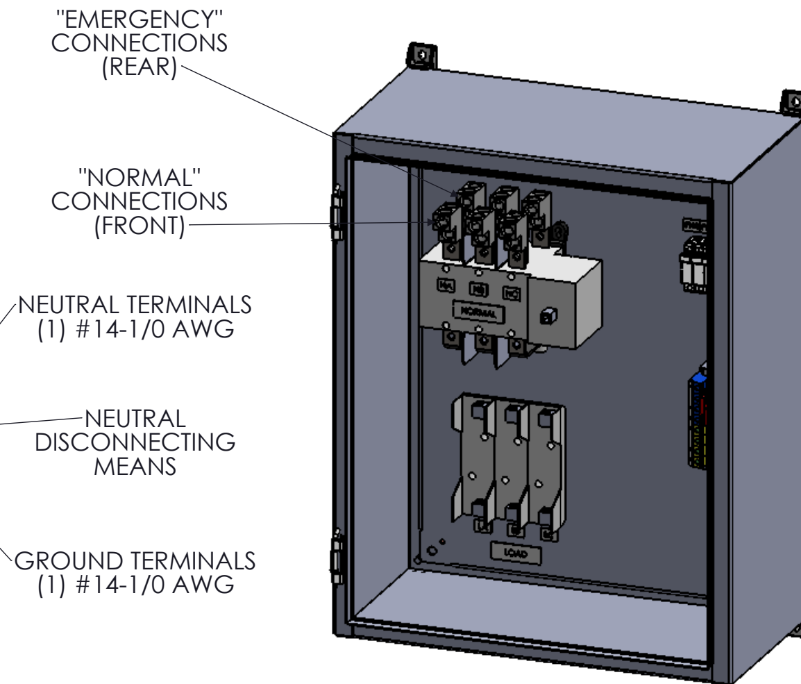
DIMETRIC VIEW DOOR REMOVED
