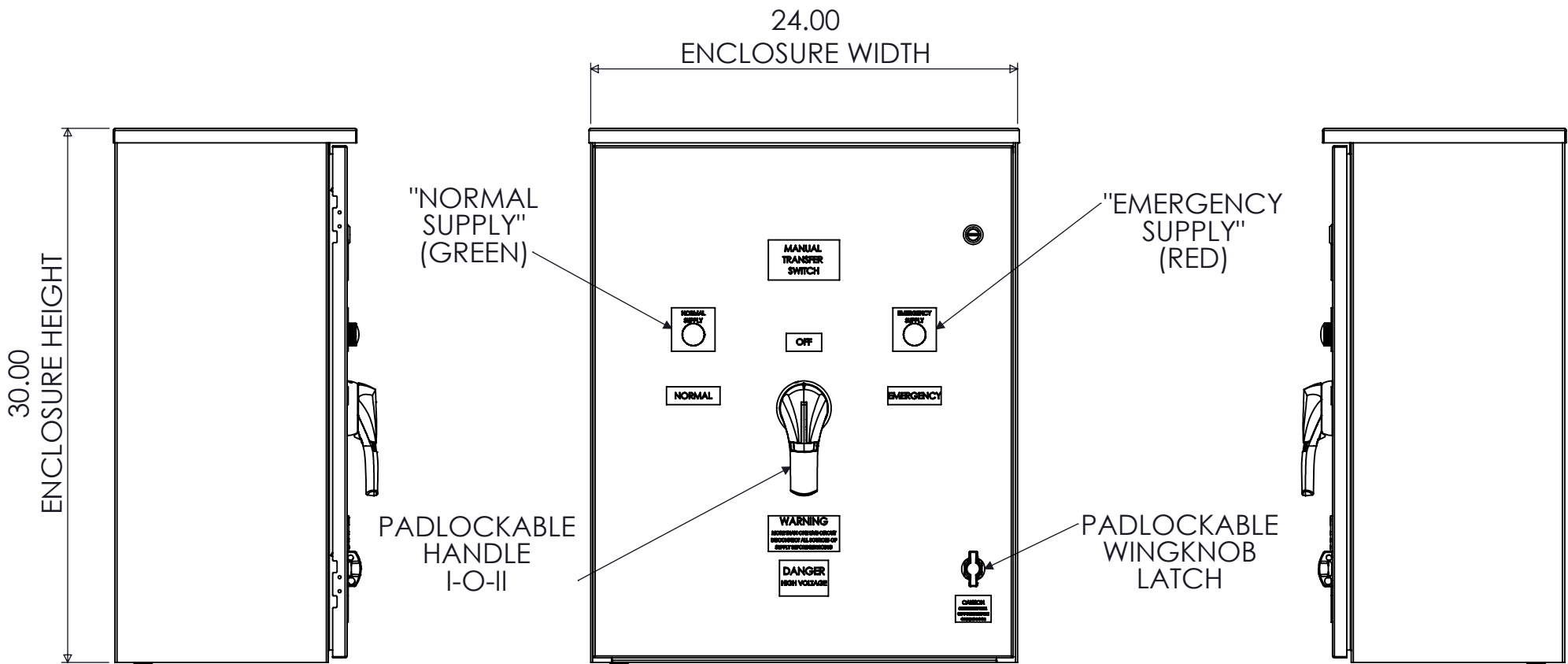
SIDE VIEW
