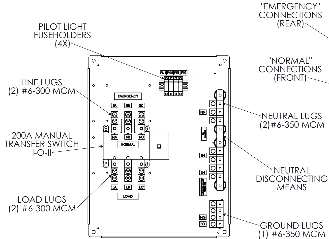
FRONT VIEW ENCLOSURE REMOVED
