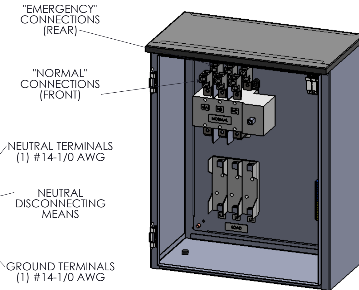
DIMETRIC VIEW DOOR REMOVED
