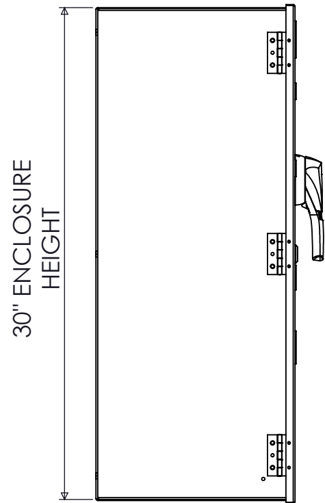
SIDE VIEW
