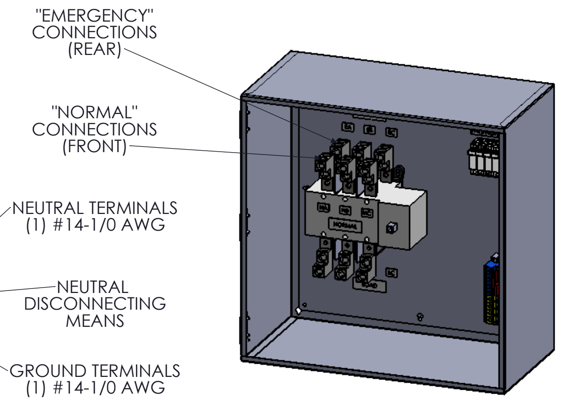
DIMETRIC VIEW DOOR REMOVED
