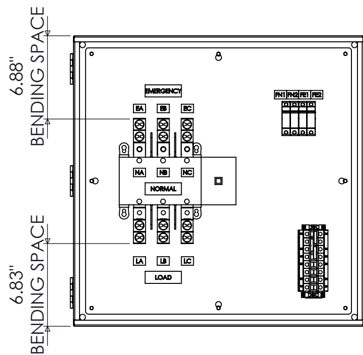
FRONT VIEW DOOR REMOVED
