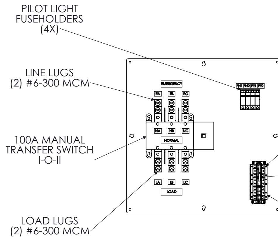
FRONT VIEW ENCLOSURE REMOVED
