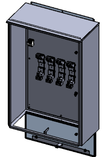
TRIMETRIC VIEW FRONT DOOR REMOVED BOTTOM DOOR OPEN
