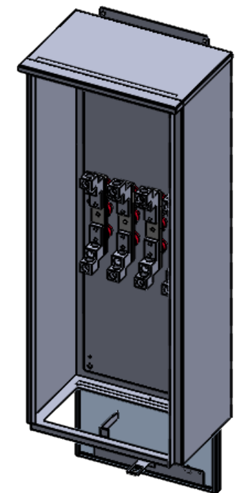
TRIMETRIC VIEW FRONT DOOR REMOVED BOTTOM DOOR OPEN
