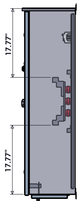
SIDE VIEW INTERIOR
