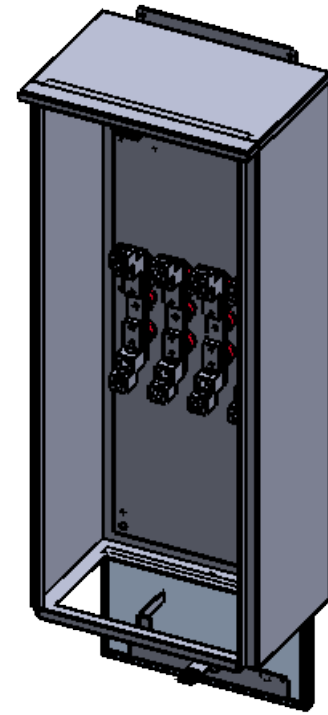
TRIMETRIC VIEW FRONT DOOR REMOVED BOTTOM DOOR OPEN
