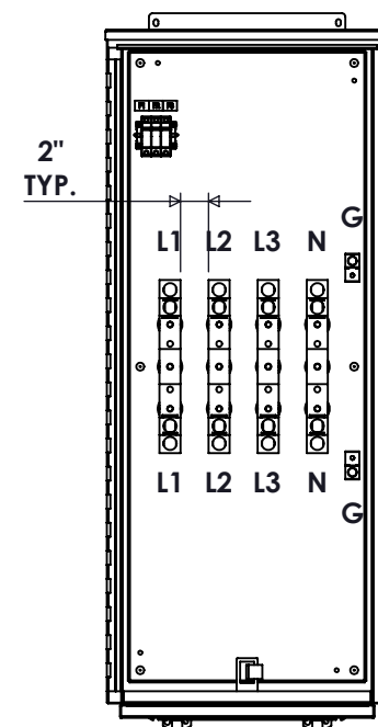
FRONT VIEW DOOR REMOVED
