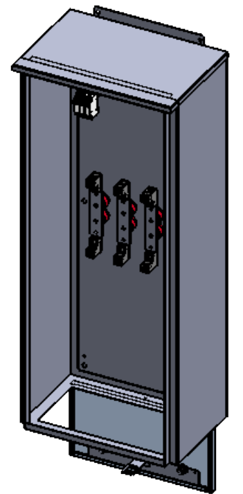
TRIMETRIC VIEW FRONT DOOR REMOVED BOTTOM DOOR OPEN
