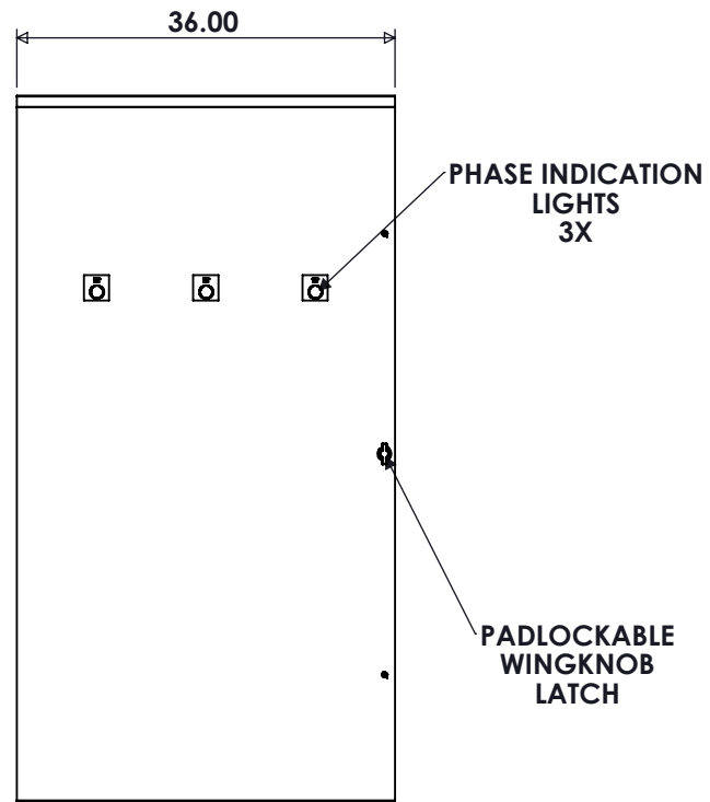
FRONT VIEW
