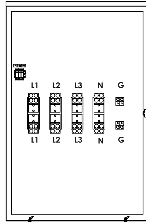
FRONT VIEW DOOR REMOVED
