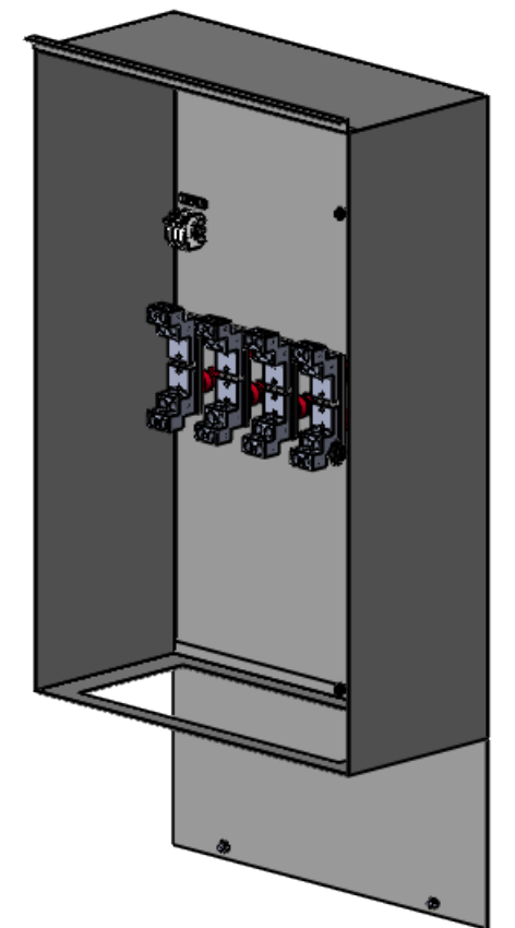
DIMETRIC VIEW FRONT DOOR REMOVED BOTTOM DOOR OPEN
